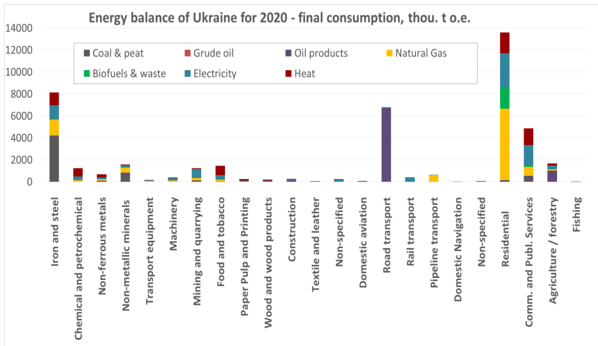
Fig.6. Energy balance of Ukraine. Final energy consumption in 2020, ktoe
