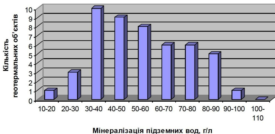
Fig. 32. Underground mineralization distribution in the geothermal objects of the the Black Sea artesian basin [30].
