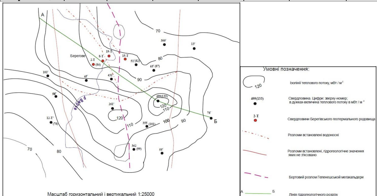
Fig. 34. Map diagram of heat flows and basic geological structures.
