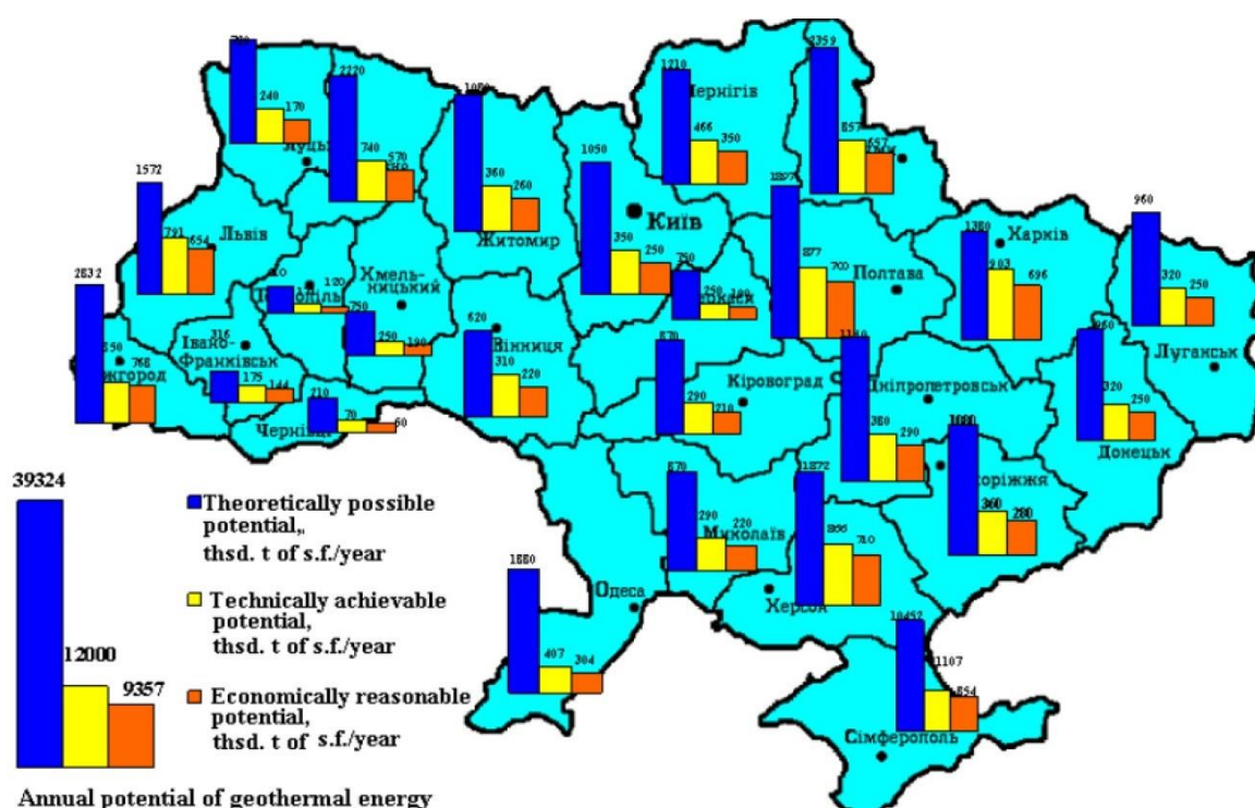
Fig. 1. Distribution of geothermal energy potential in Ukraine [24]
