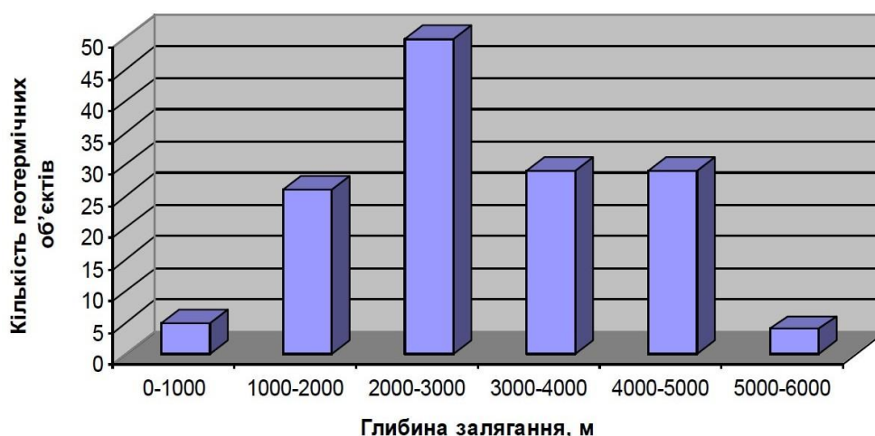
Fig. 27. Aquifer depth distributions in geothermal the objects of the Dnieper-Donetsk artesian basin.
