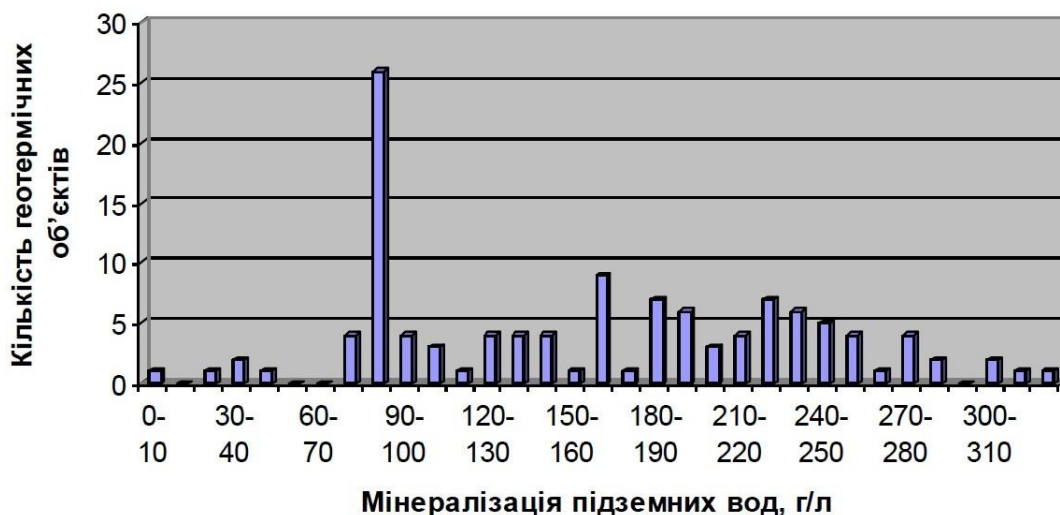
Fig. 29. Underground mineralization distribution in the geothermal objects of the Dnieper-Donetsk artesian basin.
