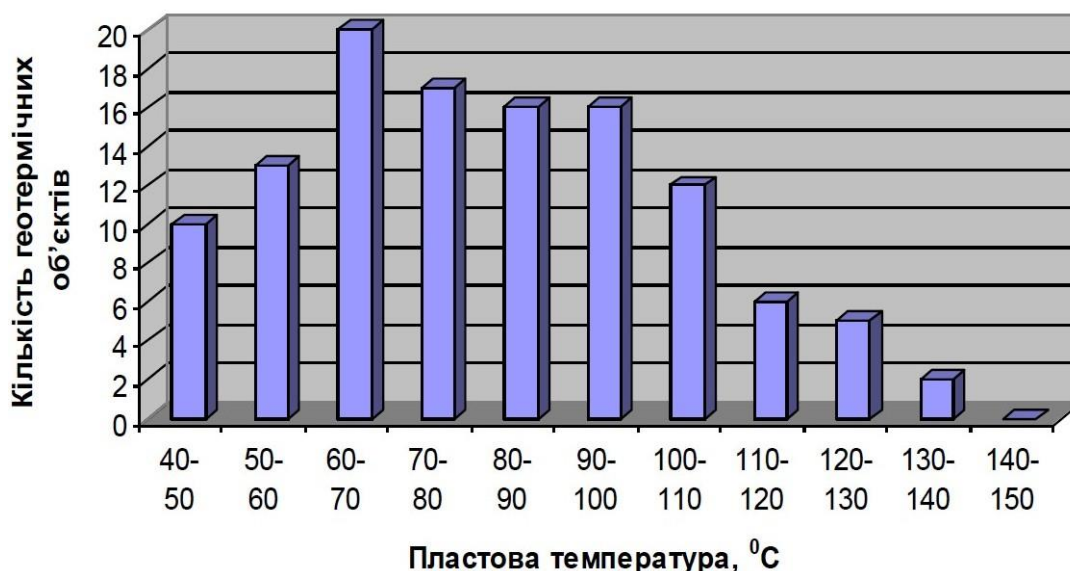
Fig. 28. Aquifer reservoir temperatures distribution in the geothermal objects of the Dnieper-Donetsk artesian basin.
