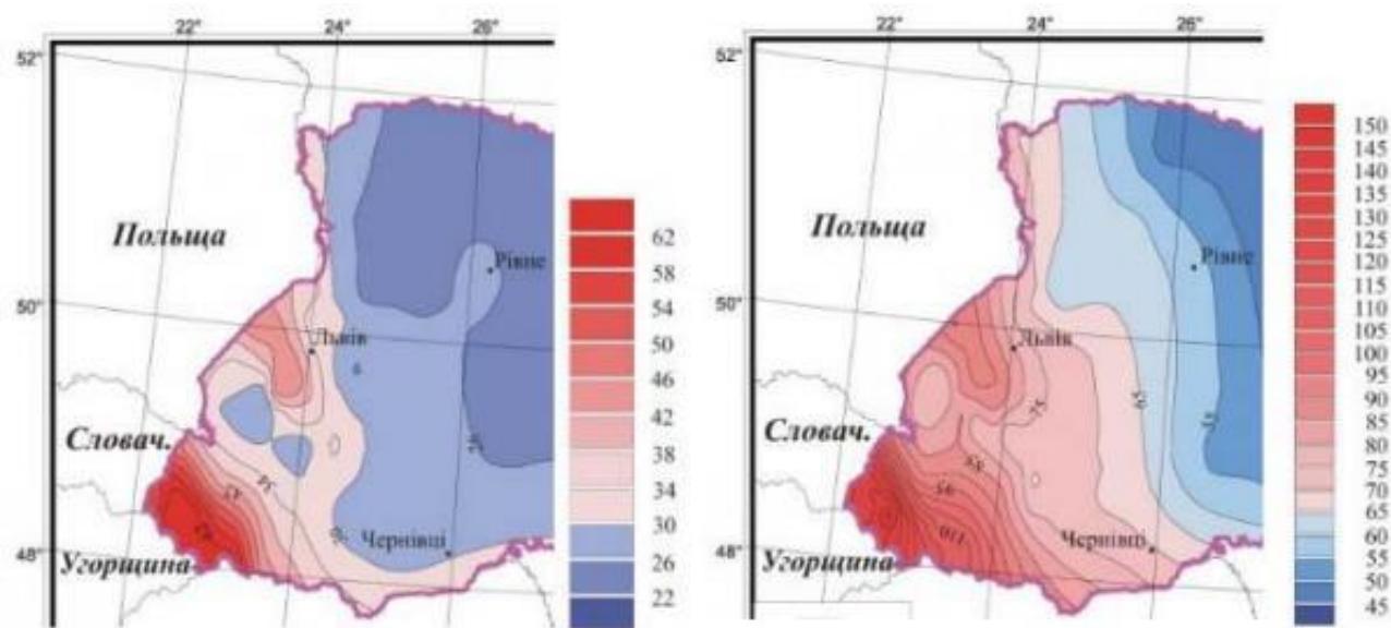
Fig. 16. Temperature map at 1,000 m (left) and 3,000 m (right) depth [26]
