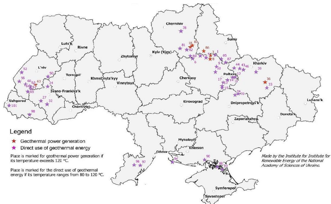
Fig. 18. The location of some promising places for the use of geothermal energy in Ukraine [24]
