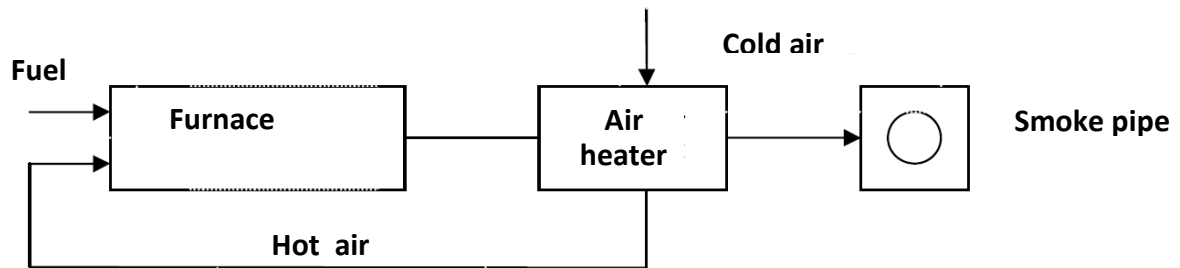
Fig. 9. Closed diagram for heat recovery of waste gases
