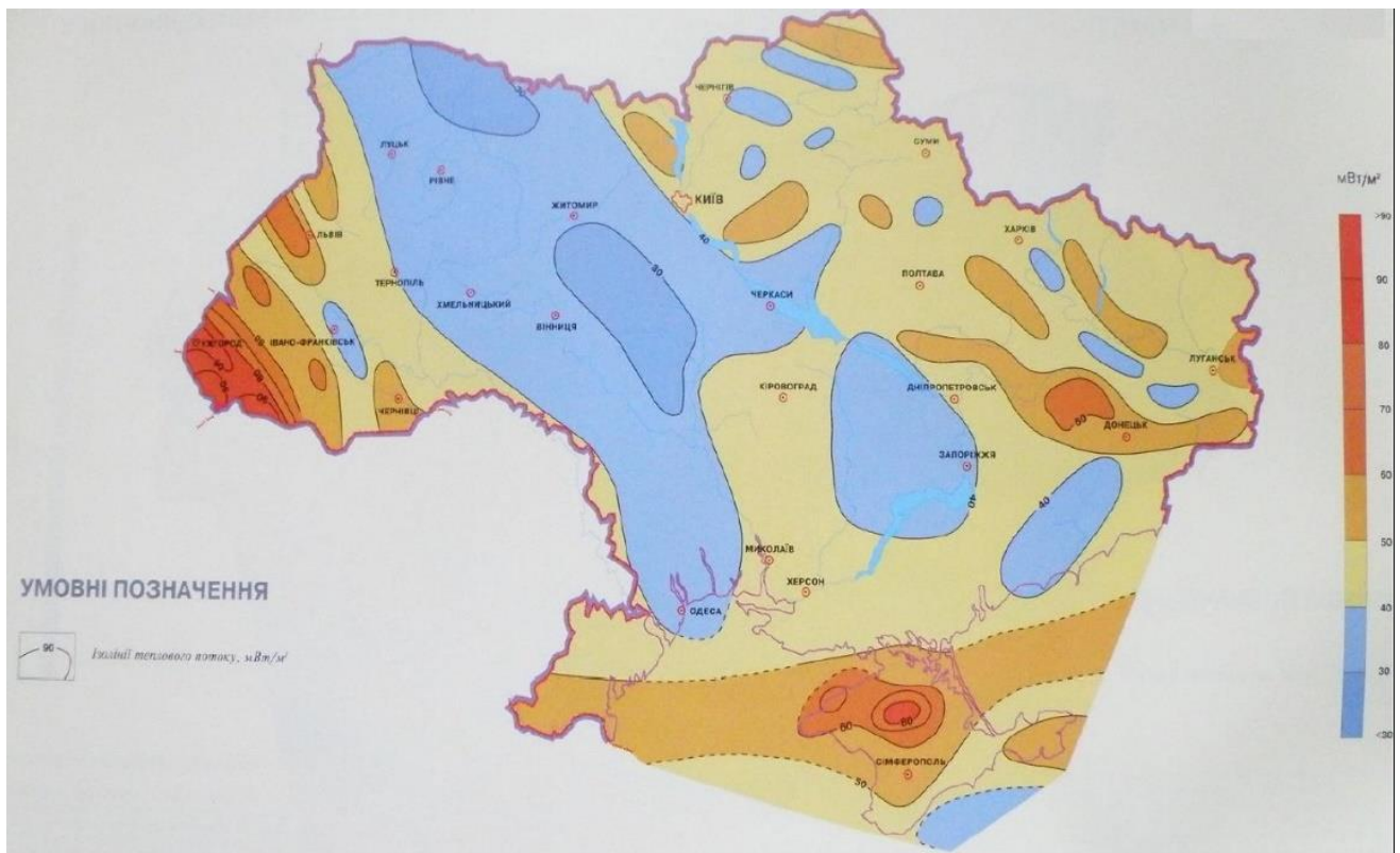
Fig. 20. Distribution of deep heat flux values on the territory of Ukraine, \text{mW/m}^2
