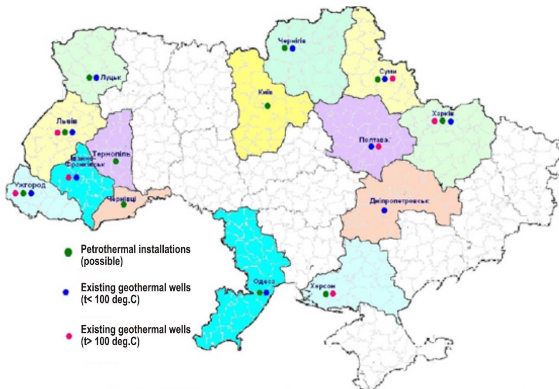
Fig. 17. Promising regions of Ukraine for the development of geothermal energy [23]
