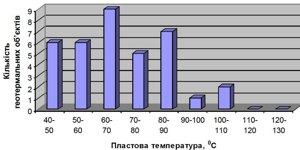
Fig. 31. Aquifer reservoir temperatures distribution in the geothermal objects of the Black Sea artesian basin.
