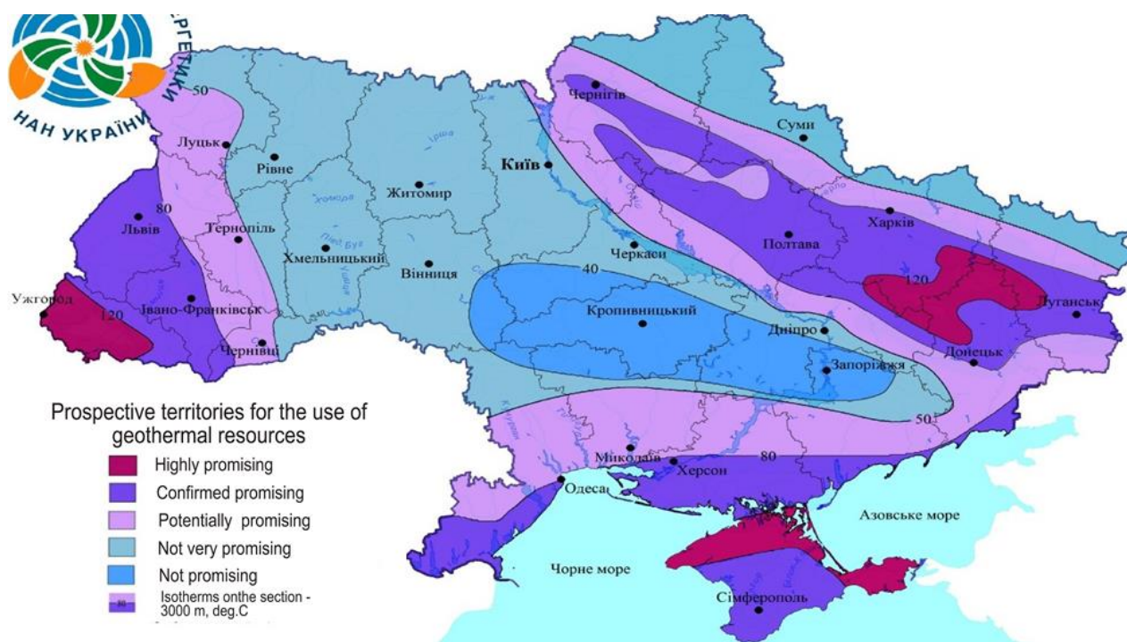
Fig. 14. Prospective territories for the use of geothermal resources [22]
