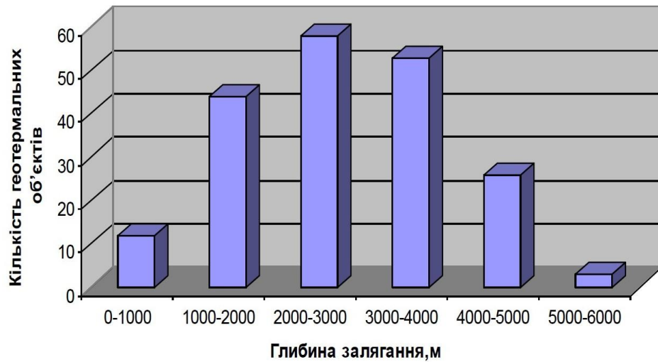
Fig. 2. Aquifer depth distributions in the geothermal objects of the Carpathian bend.
