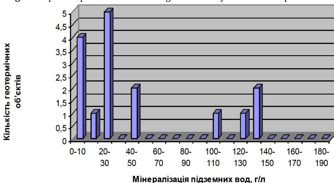
Fig. 23. Aquifer mineralization distribution in the geothermal objects of Transcarpathian bend.
