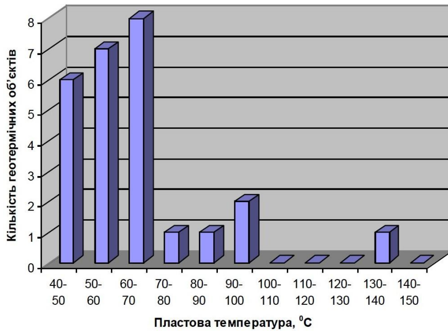
Fig. 21. Aquifer temperature distribution in the geothermal objects of Transcarpathian bend.
