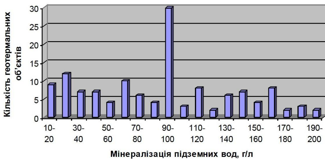
Fig. 26. Underground mineralization distribution in the geothermal objects of the Carpathian bend.
