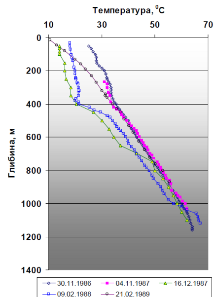
Fig. 37. Temperature distribution in well № 19-T during experimental filtering works.
