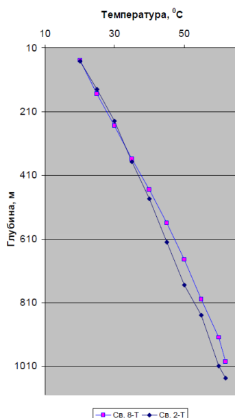
Fig. 35. Distribution of temperature in operational wells after drilling.
