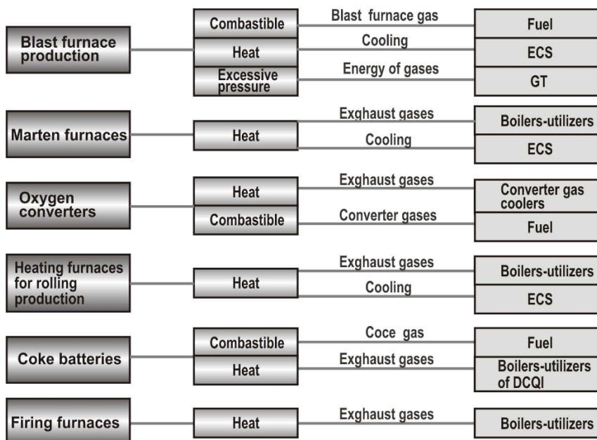
Fig. 8. The structure of production and disposal of WE in ferrous metallurgy [8].
