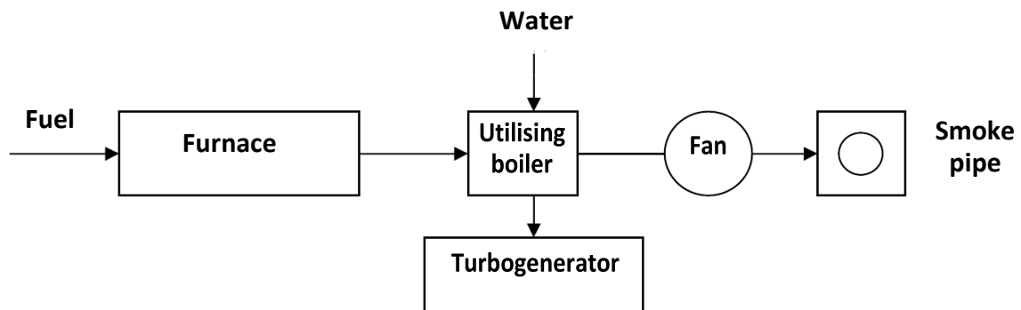
Fig. 10. Open diagram of heat recovery of waste gases
