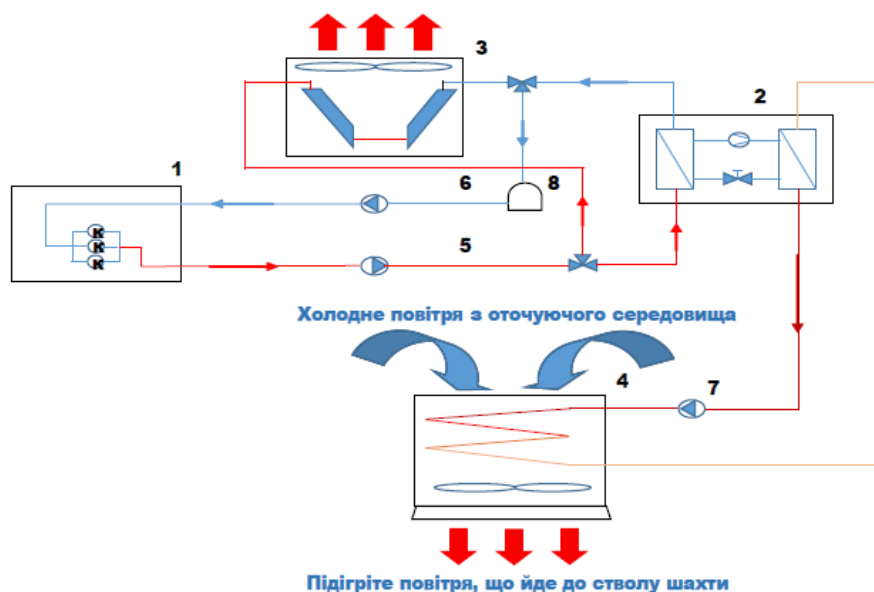
1 – compressor station, 2 – heat pump station, 3 – cooling tower, 4 – heat exchanger for heating the air supplied to the shaft of the mine, 5, 6, 7 – circulation pumps, 8 – hydromodule.
