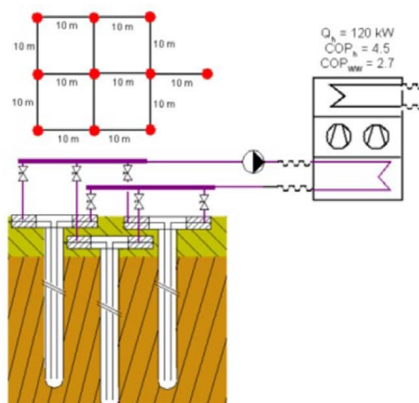
Fig. 40. Recommended location of 10 probes on a geothermal field for heat supply of an apartment building
