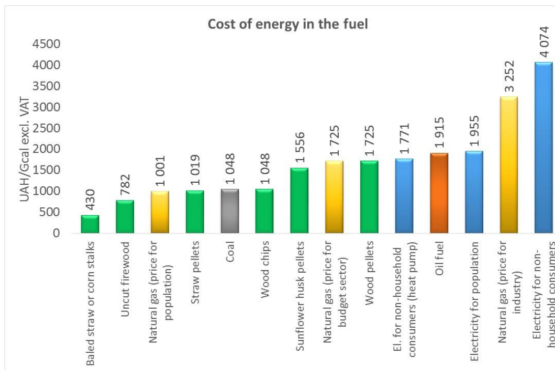
Fig. 4 Cost of energy in the fuel (of heating season 2021-2022)
