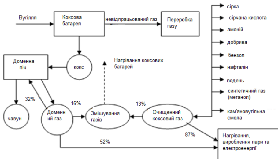
Fig. 7. The scheme of coke production, integrated to the metallurgical enterprise [8]
