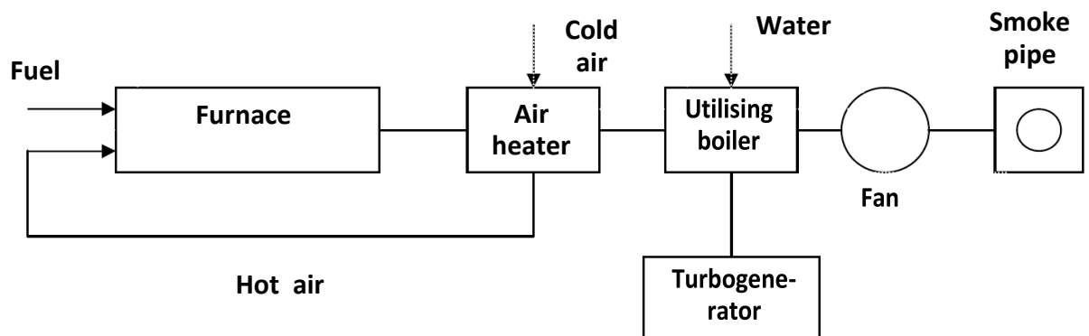
Fig. 11. Diagram of combined heat recovery of waste gases
