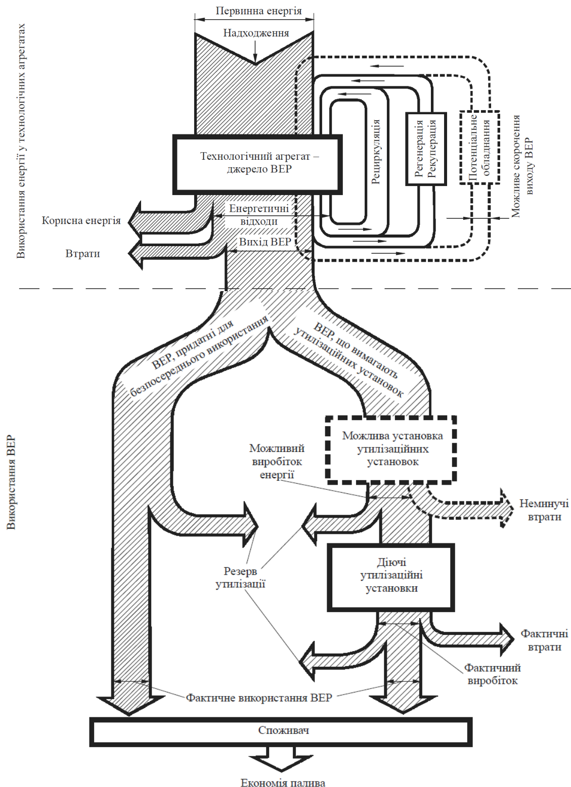
Fig. 5. Energy use flow diagram with WE recovery [4].
