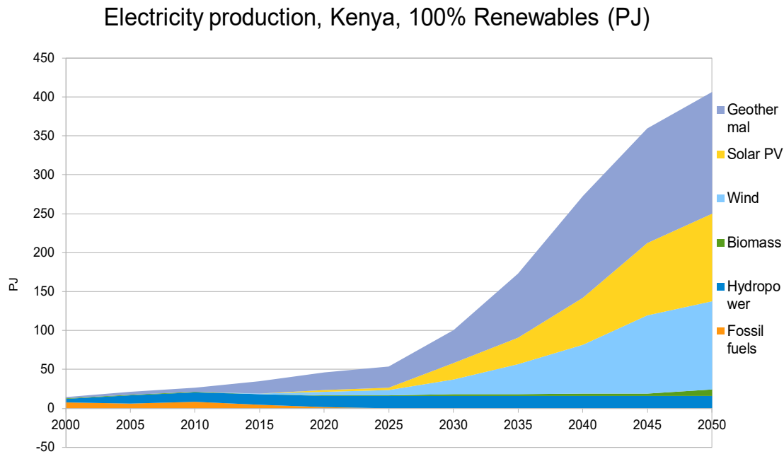
Graph 11. Electricity production in the 100 % renewable-energy scenario.
