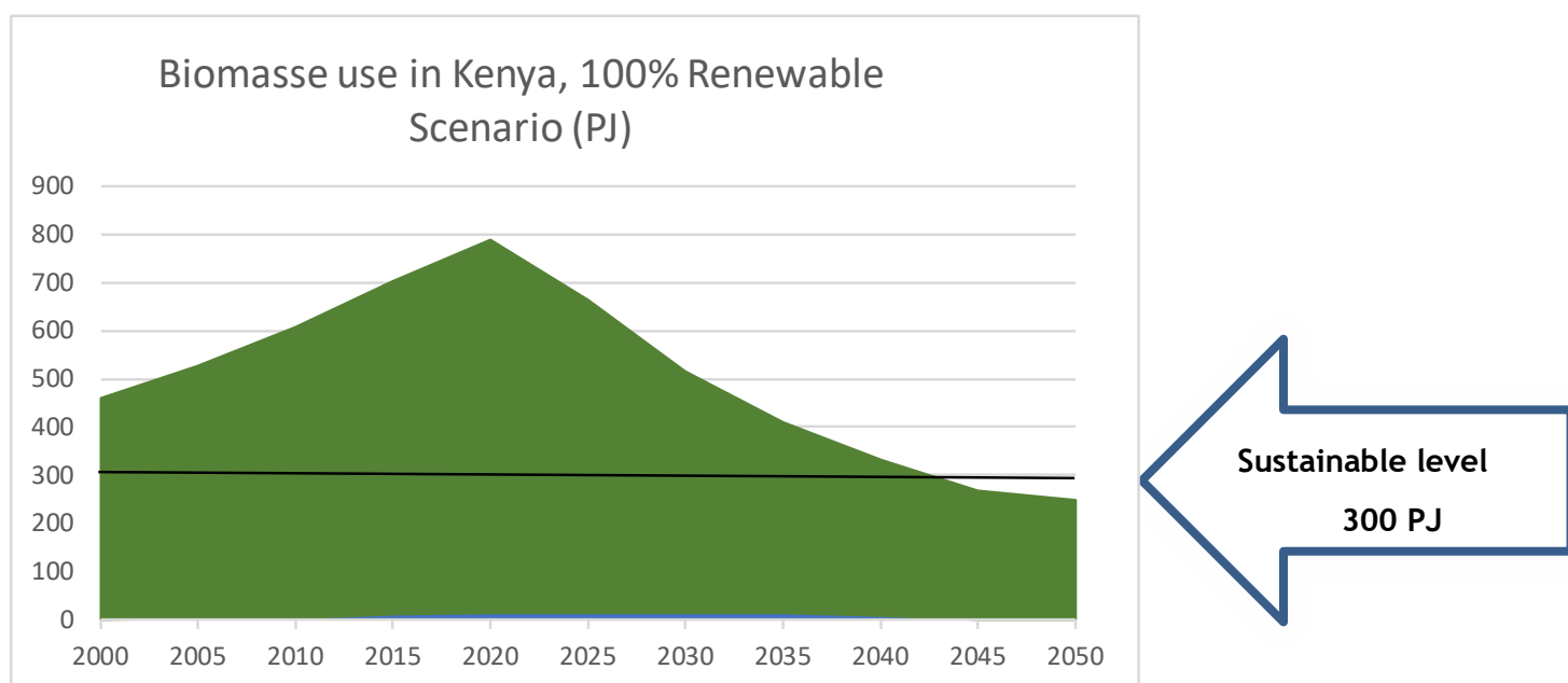
Graph 13. Biomass use (all) in 100% renewable-energy scenario.
