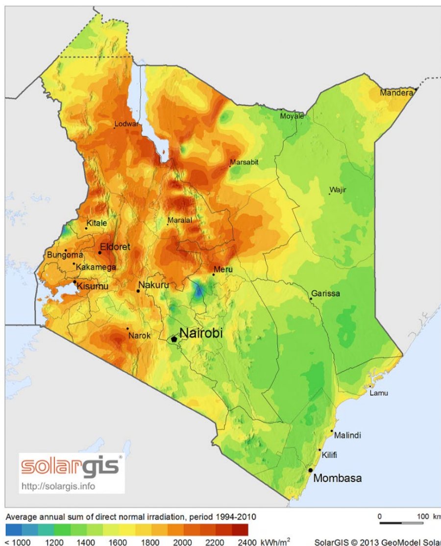
Figure 3 Map showing direct solar irradiation in Kenya
