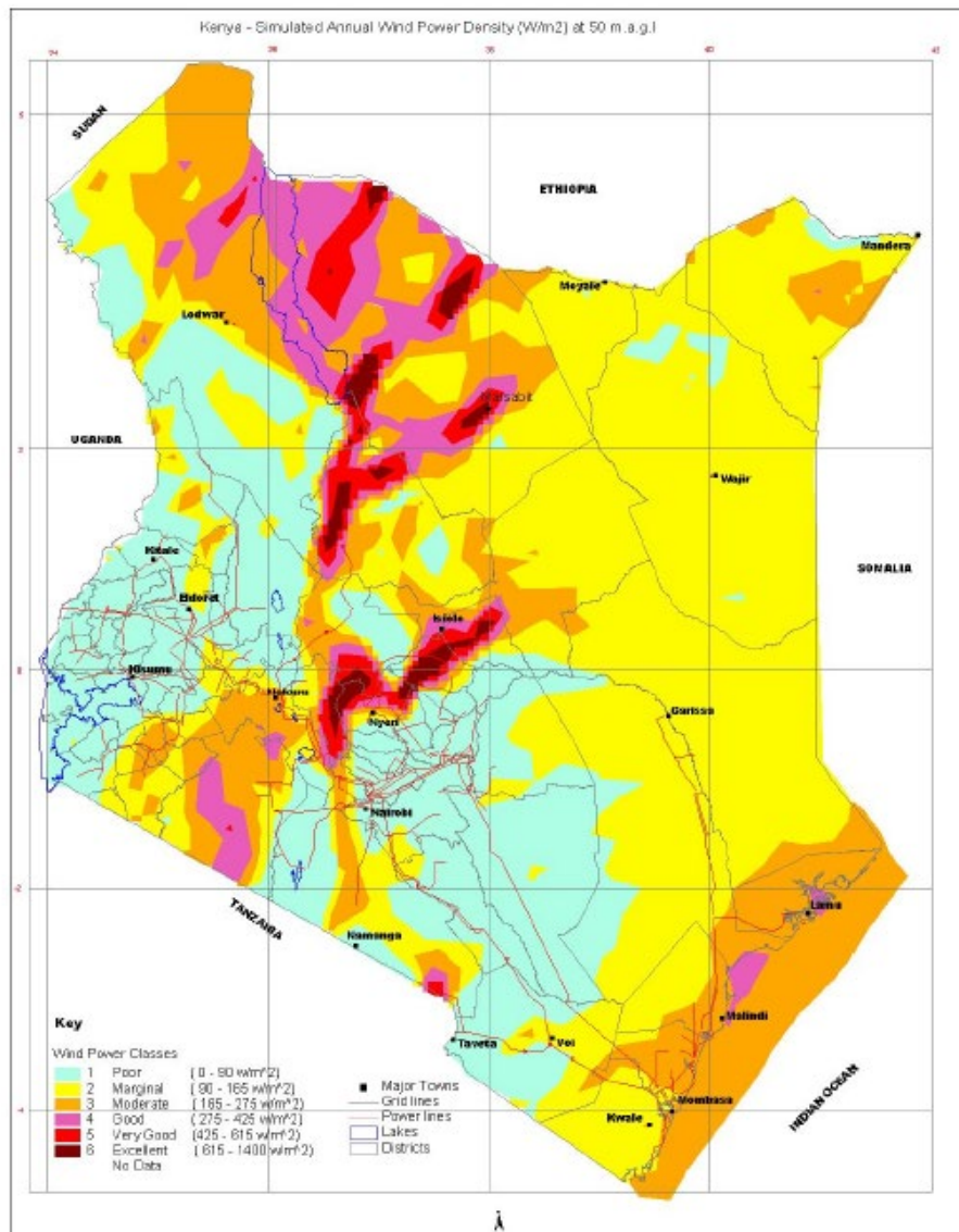
Figure 2: The Map showing standard wind power density at 50 m above ground in Kenya
