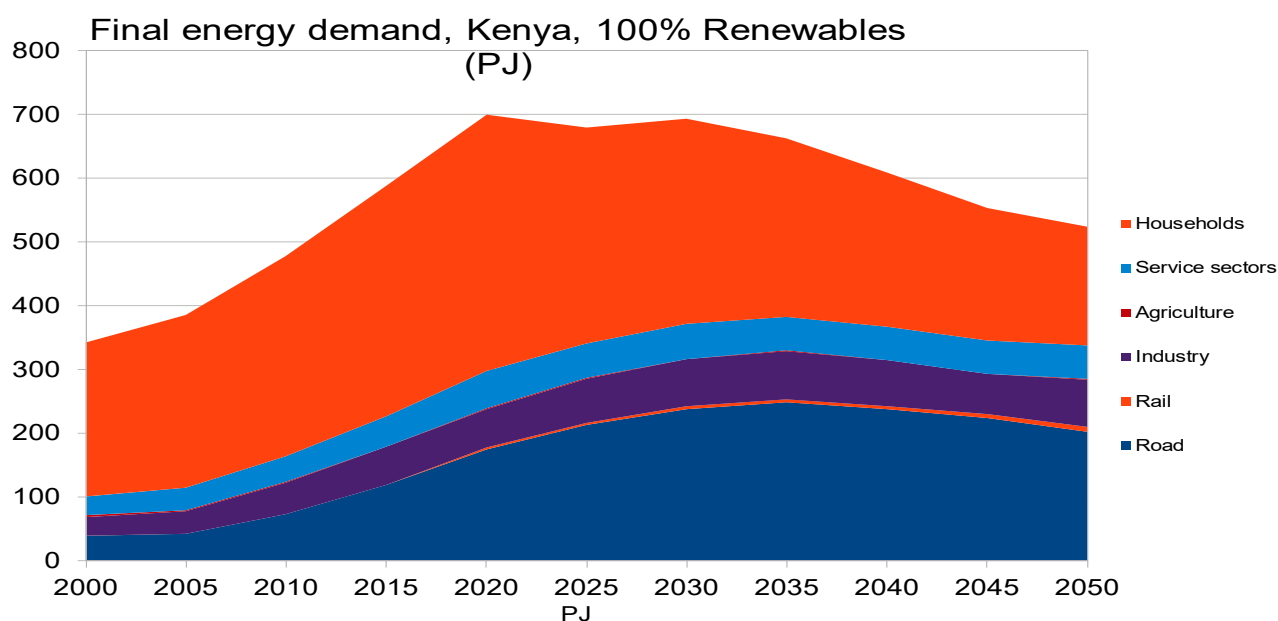
Graph 4. Final energy demand in the 100 % Renewable Energy Scenario, based on assumptions in this chapter and in Annex 1.
