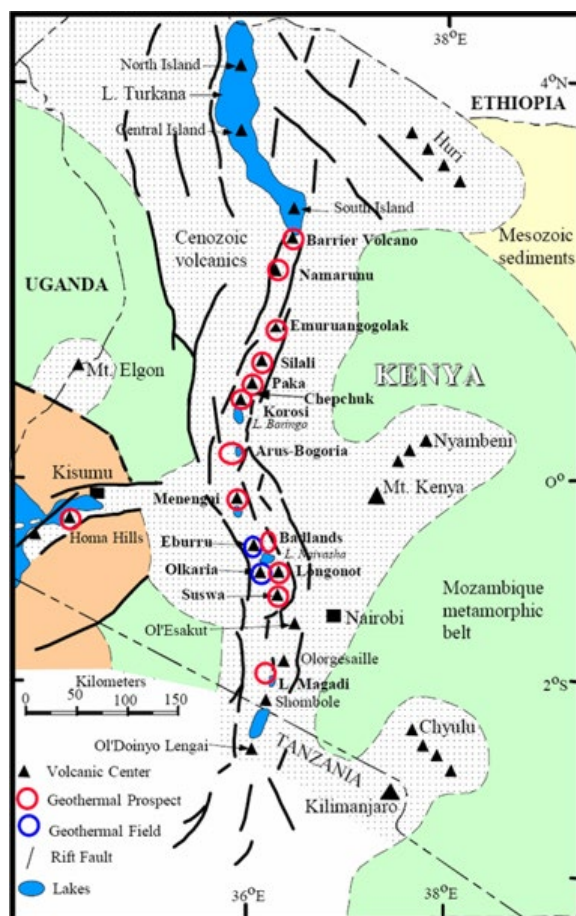
Figure 4: Geothermal prospect locations in Kenya, Source: EPRA, 2020
